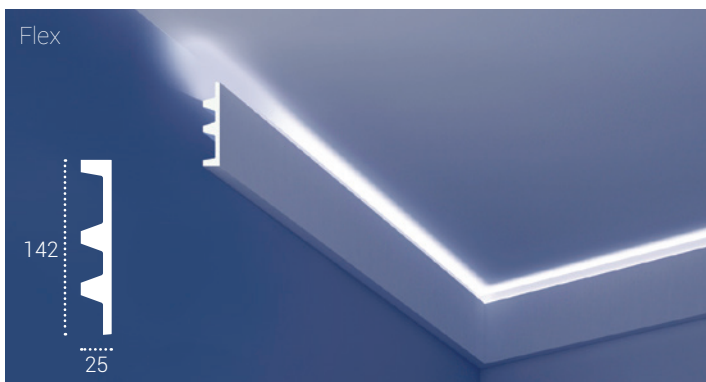
KF 505 | 142x25mm
