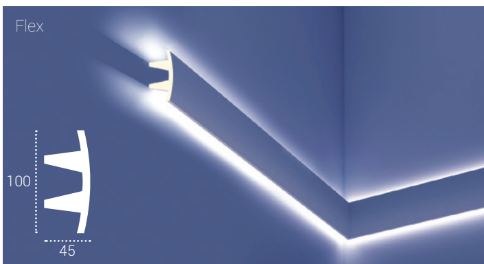
KF 503 | 100x45mm
